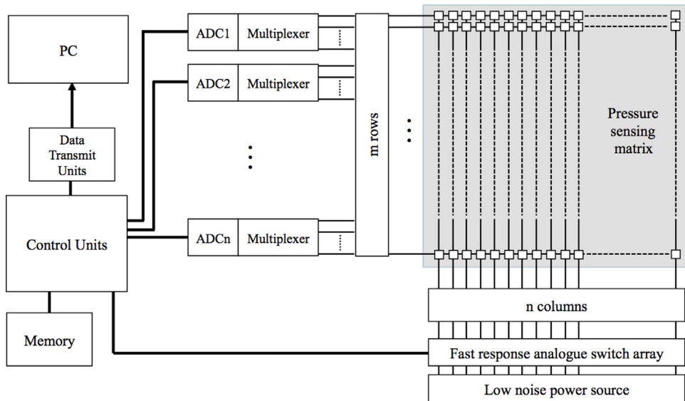
Fig. 2. System architecture.
